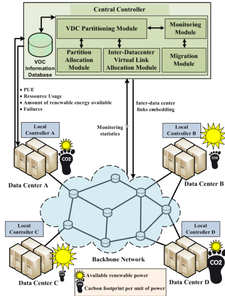
Fig. 1: Proposed framework
